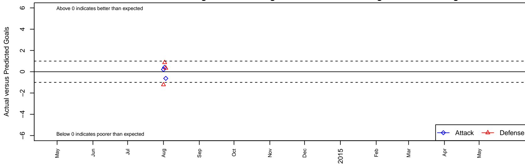
Kitsap Pumas –Unk2 B00 Dots are actual minus expected GF (blue circles) and GA (red triangles). Blue line is smoothed change in attack strength. Red is smoothed change in defense strength.
